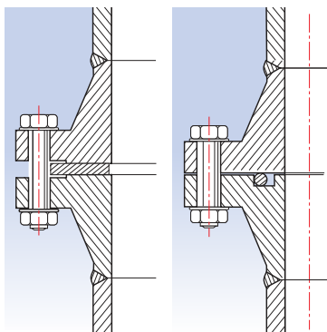
‘FLOATING’ ASSEMBLY
